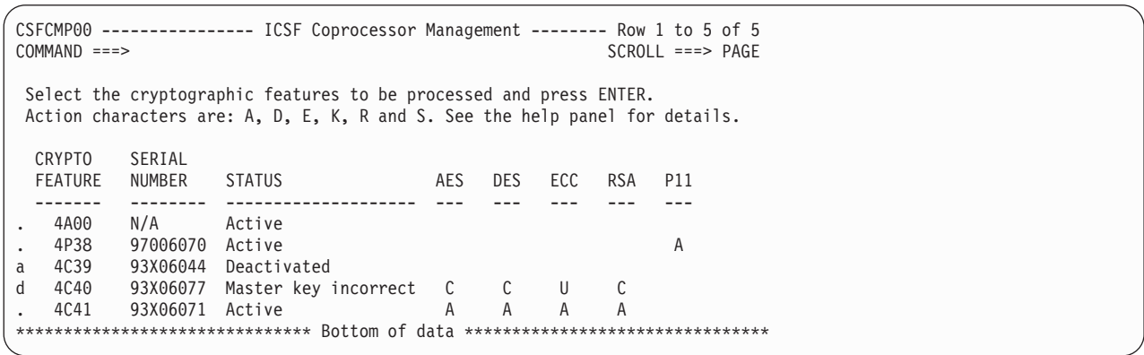
Figure 2. ICSF coprocessor management
